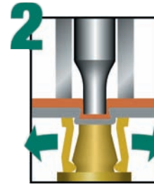
2 The punch pushes the material into the die which opens and forms a ‘mushroom’ lock.
