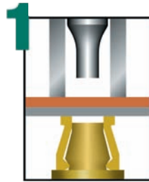
1 The tooling clamps the material between the punch and die.
