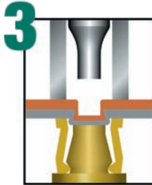
3 The punch is stripped out and the lock remains.
