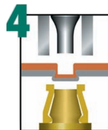
4 The tooling unclamps the material and the part is easily removed.
